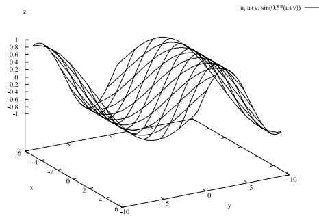
Fig. 15. splot u,u+v,sin(0.5*(u+v))
