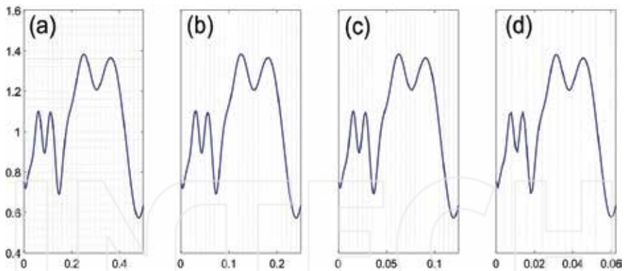
Figure 18. Spatial distribution of the acoustic pressure level (in dB) along the Z -axis for the PCFL with D = 0.6 , N = 5 , f_{gc} = 0.4 , s = 2 for (a) R = 12.5 cm, (b) R = 6.25 cm, (c) R = 3.125 cm, and (d) R = 1.5625 cm.
