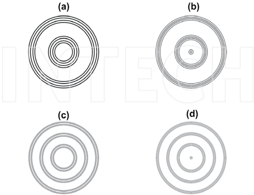
Figure 16. XY-plane view of the PCFL with f_{gc} = 0.4 , D = 0.6 , s = 2 , and R = 12.5 cm and f = 100 kHz for (a) N = 4 , (b) N = 5 , (c) N = 6 , and (d) N = 7 .
