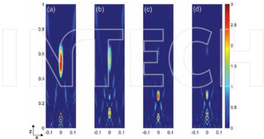
Figure 17. Two-dimensional spatial distribution of the acoustic gain (in dB) in the XZ-plane for the PCFL with f_{gc} = 0.4 , D = 0.6 , s = 2 , and R = 12.5 cm parameters and working frequency of 100 kHz. The number of solid zones is: (a) N = 4 , (b) N = 5 , (c) N = 6 , and (d) N = 7 .
