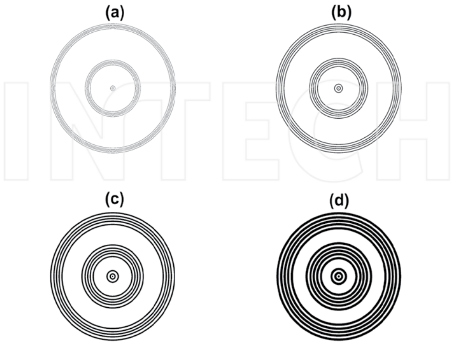
Figure 12. XY-plane view of the PCFL with N=5 , f_{gc}=0.4 , s=2 , and R=12.5 cm and f=100 kHz for: (a) D=0.5 , (b) D=0.6 , (c) D=0.7 , and (d) D=0.8 .
