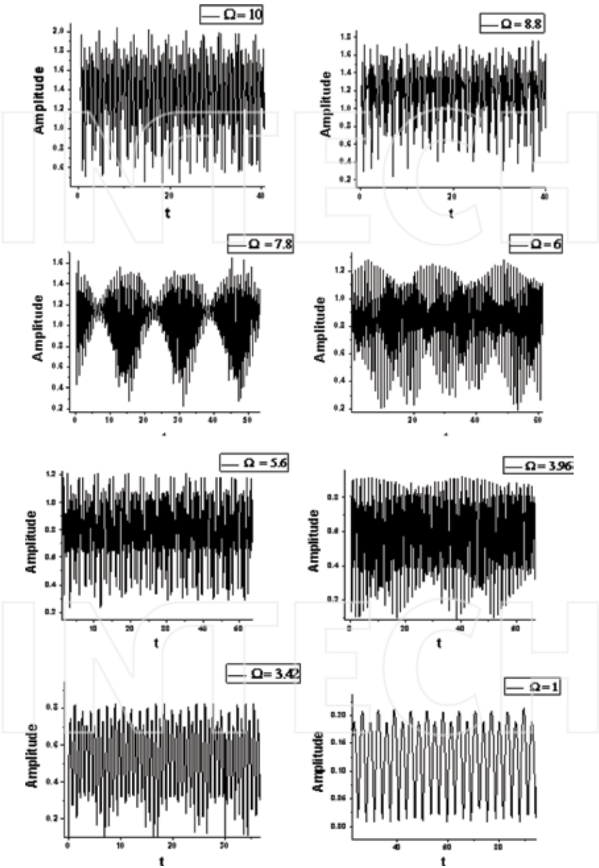
Figure 19. Discharge current temporal traces for different values of the oscillation frequency at a constant damping coefficient ( r = 0.1 ).
