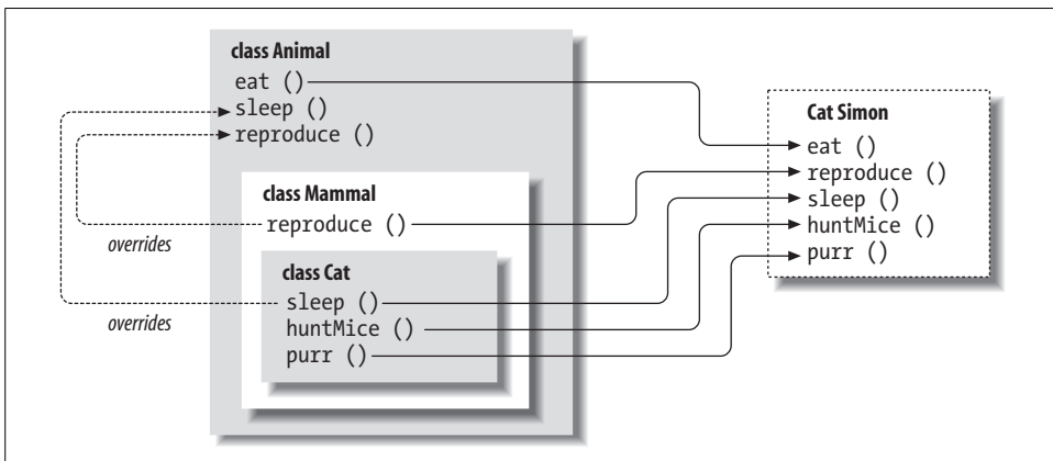
Figure 6-3. Method overriding
