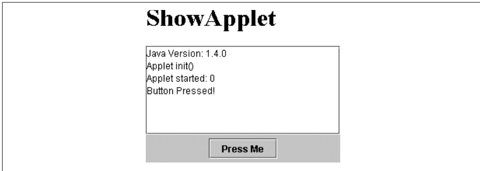
Figure 23-2. ShowApplet
