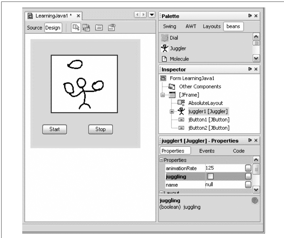
Figure 22-3. Juggling beans
