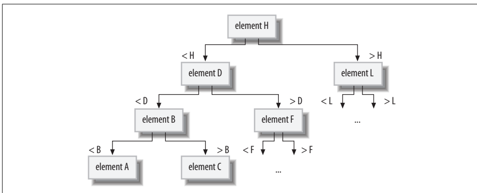
Figure 11-4. Tree structure
