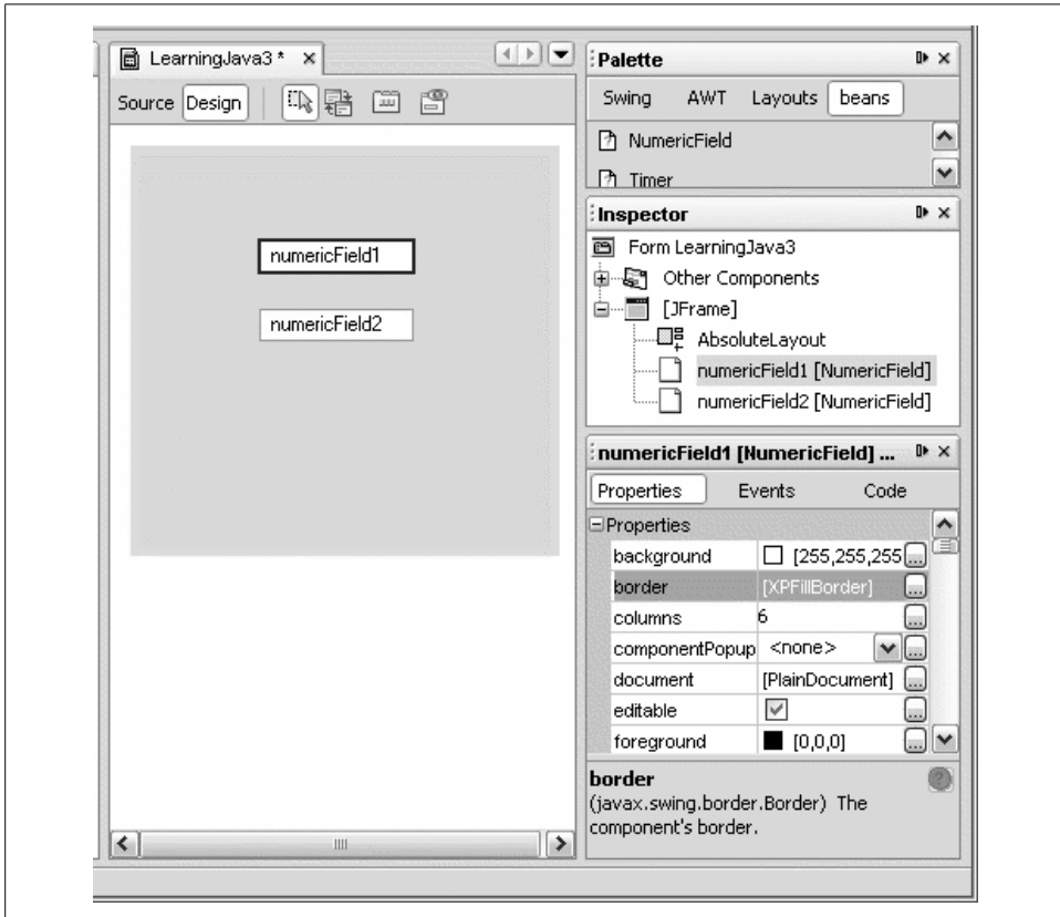
Figure 22-7. Binding properties
