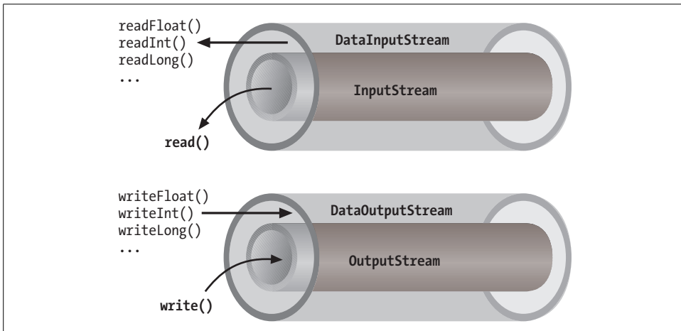
Figure 12-3. Layered streams
