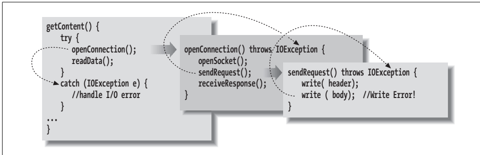
Figure 4-3. Exception propagation
