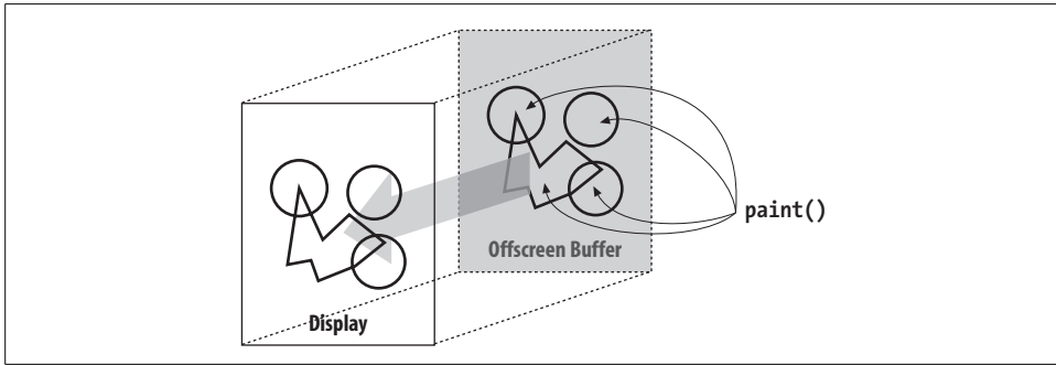
Figure 20-5. Double buffering
