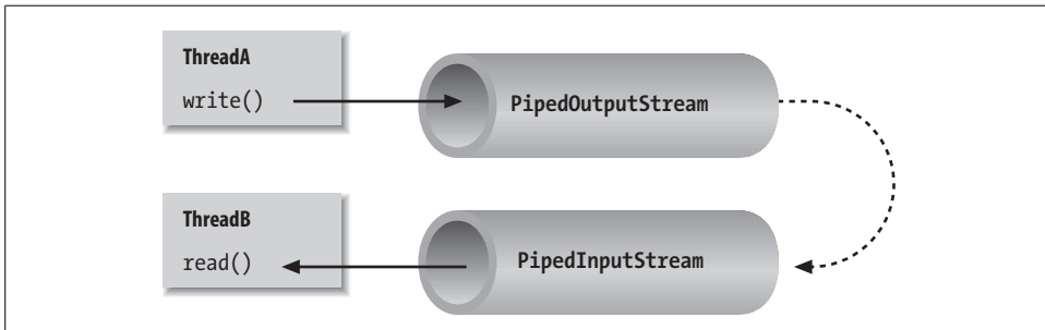
Figure 12-4. Piped streams
