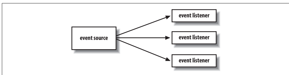
Figure 16-3. Event delivery
