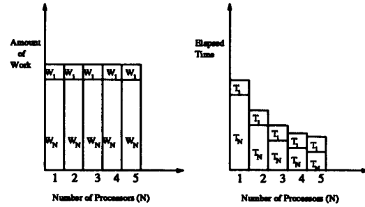
Figure 4. Amdahl's Law
